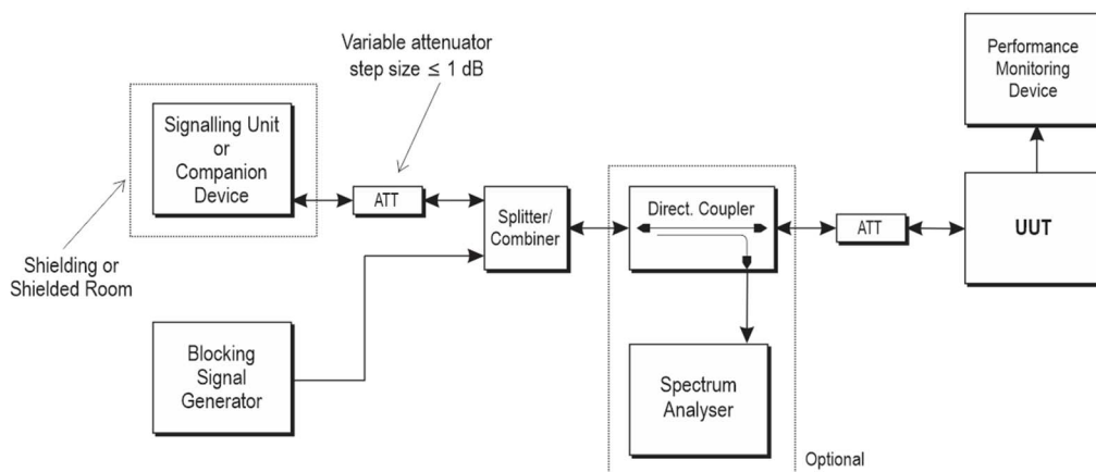
Figure 12: Test set up for receiver blocking
