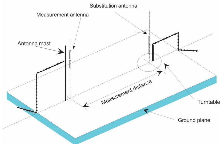
Figure B.1: A typical OATS
