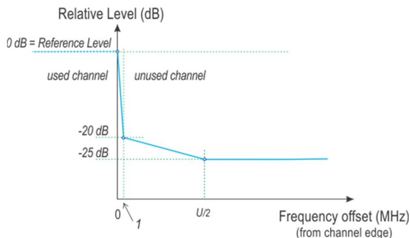
Figure 3: Channel edge mask - case 2
