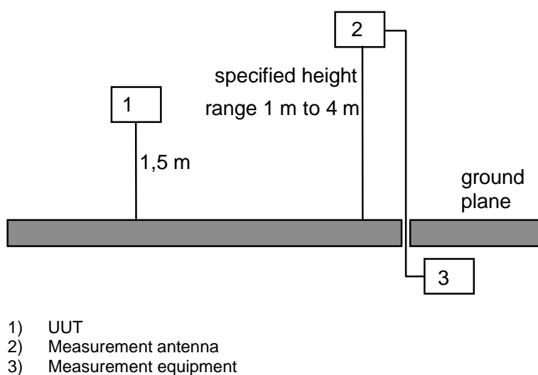
Figure C.1: Measurement arrangement for radiated measurements
