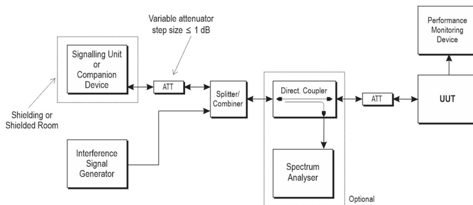
Figure 13: Test set up for receiver selectivity
