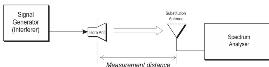
Figure C.7: Measurement set up for calibration
