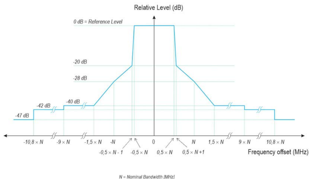
Figure 1: Transmit spectral power mask
