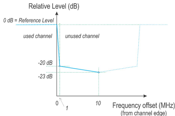
Figure 4: Channel edge mask - case 3
