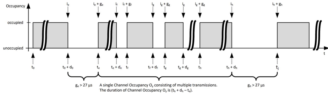
Figure 11: Example of UUT transmissions
