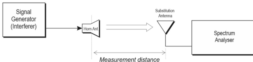
Figure C.3: Measurement set up for calibration
