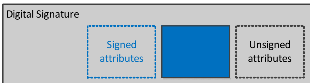
Figure 3: Digital Signature
