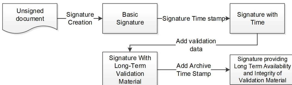
Figure 4: Signature Lifecycle
