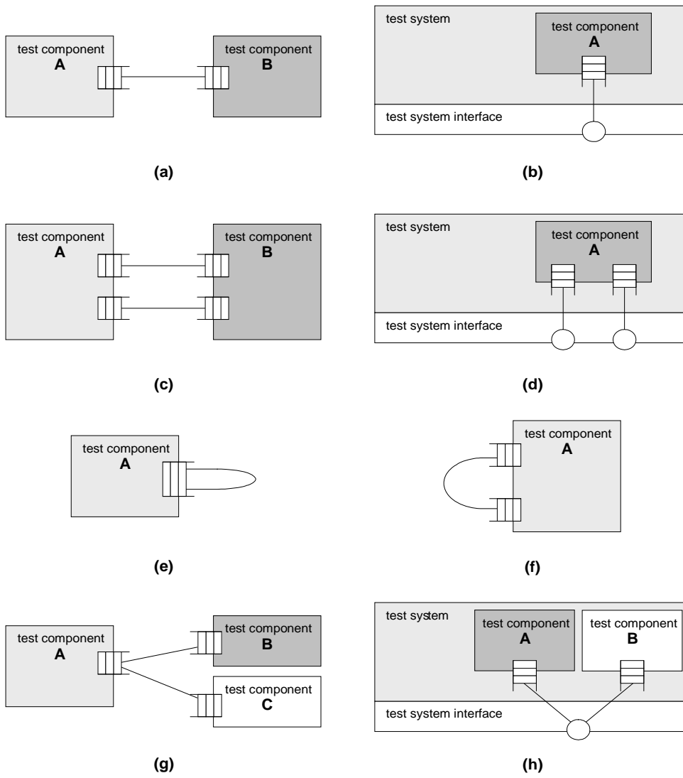
Figure 6: Allowed connections
